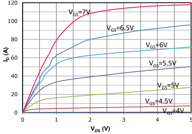
Fig 1: Output Characteristics
